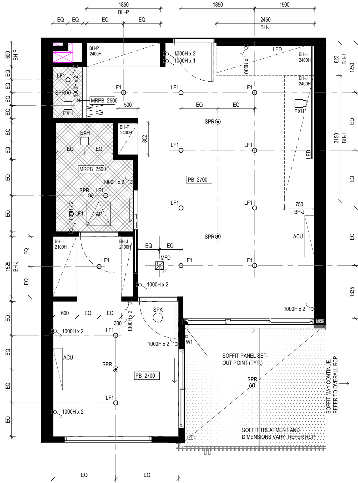
2 ILA_Type 1 RCP Scale 1:50 NOTE: REFER TO ELECTRICAL ENGINEER DRAWINGS FOR TYPICAL LIGHTING/CEILING SERVICES LOCATIONS & SPECIFICATION.
